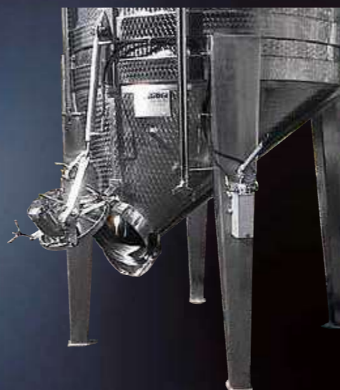
Side view of Gravitank with door open, hydraulic opening
