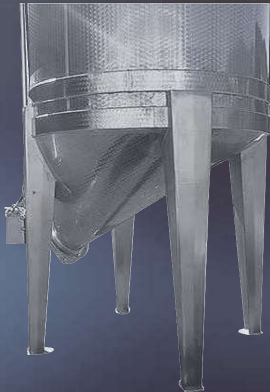
Rear view of a Gravitank with inclined tapered bottom offset towards the front
